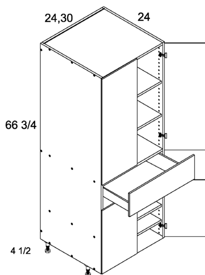
Tall Two Door Two Drawer Utility
