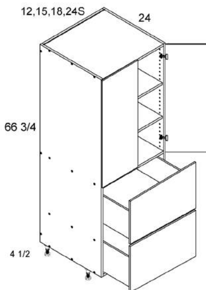
Tall Two Door Two Drawer Utility
