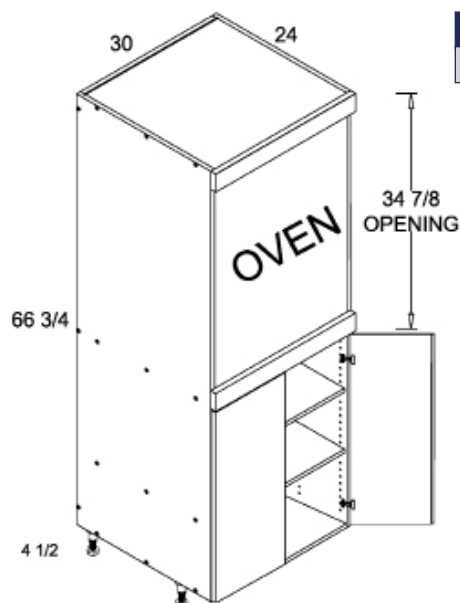
Tall Single Oven Full Height Two Door Utility
