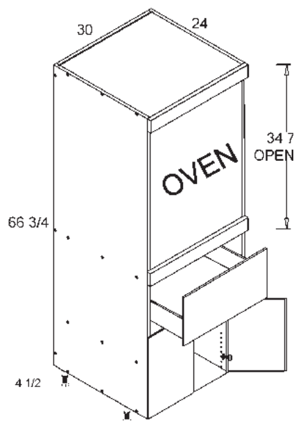
Tall Single Oven Two Door One Drawer Utility
