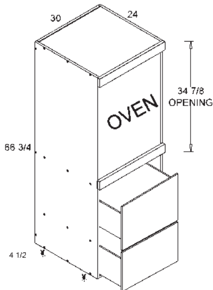
Tall Single Oven Three Drawer Utility
